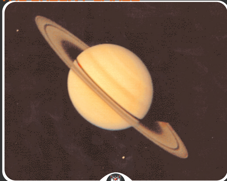
Saturn
