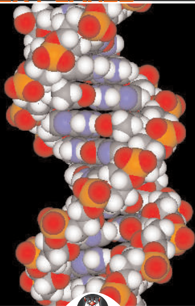
DNA
